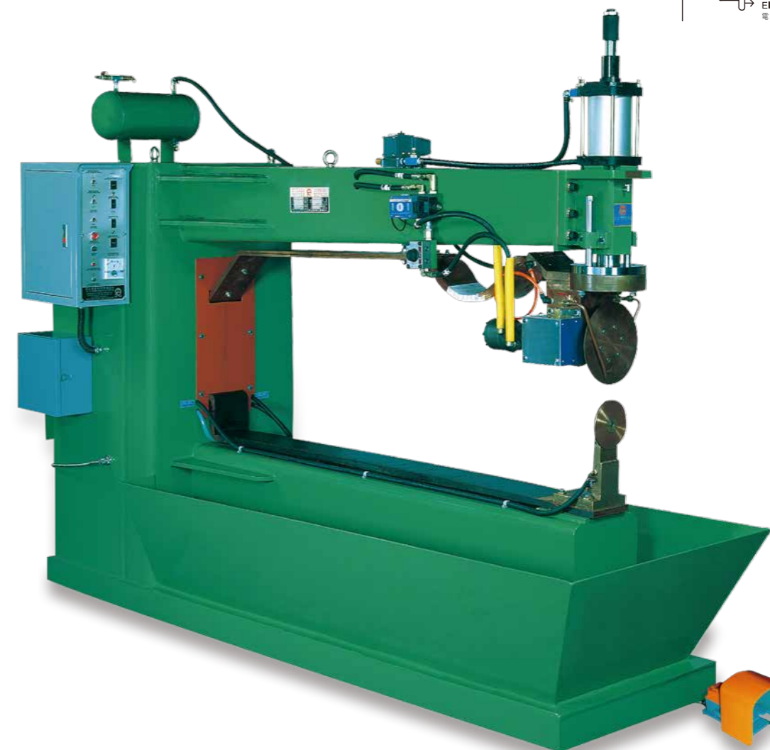
Air Hydraulic Pressure Automatic Seam Welder(Sink)
