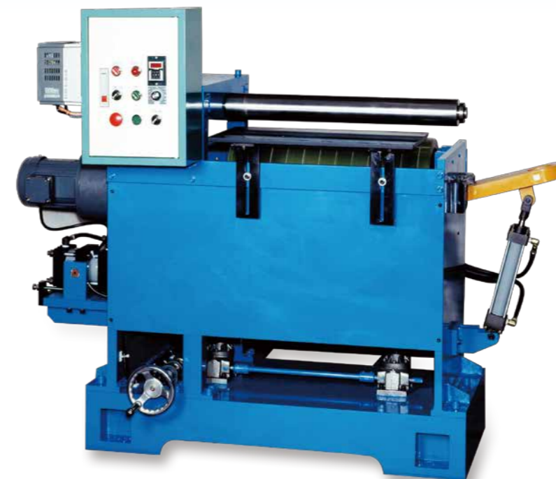
DJ-R 300~1000 Double Roller Type Bending Machine (for sheet)
