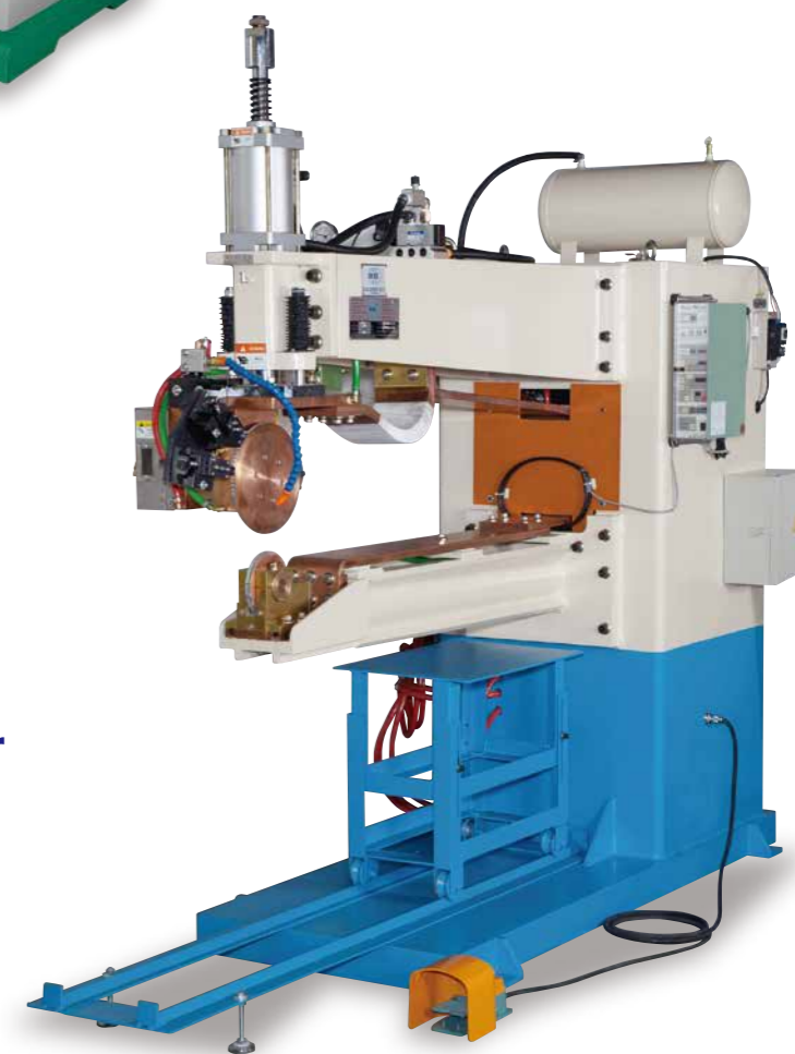
Air Hydraulic Pressure Automatic Seam Welder (Straight Line Type) 自動空油壓直線輪焊機
