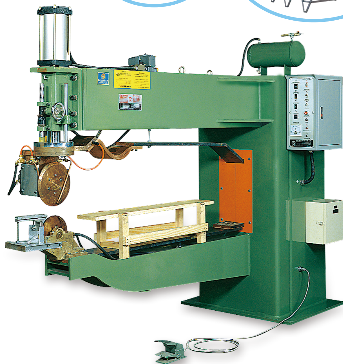
Vertical Seam Welder for Water Tank Body
