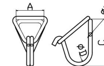
Hook and Keeper J-Hook-11
