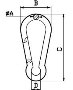
Snap Hook SNAP HOOK-02
