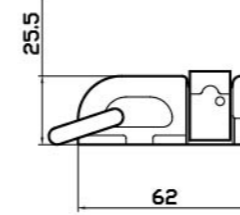
Double Stud Fitting with O ring SF202-062018025TZ-O
