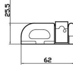
Double Stud Fitting SF202P-062018025
