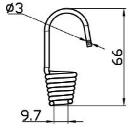
Bungee Hook-01 SPR02 SUS304
