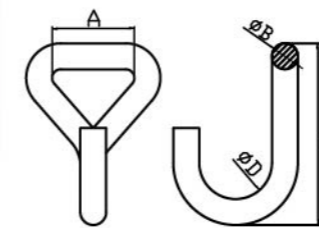
J Hook J-Hook-10
