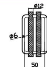
Buckle with Dual Anti-slip Adjuster Buckle-03 SUS 304
