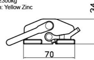
Forged End Fitting EF103-02540127061Y
