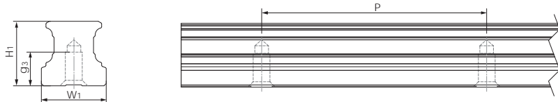
ARU Series 下鎖式滑軌
