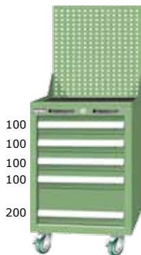
EA-7053MA H1380xW566xD640 EB-7053MA H1380xW718xD640
