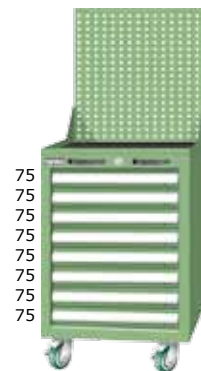
EA-7081MA H1380xW566xD640 EB-7081MA H1380xW718xD640
