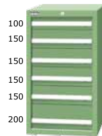
EA-10062 H1000xW566xD607 EB-10062 H1000xW718xD607 ED-10062 H1000xW718xD759
