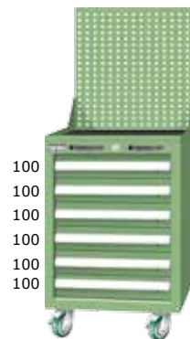
EA-7061MA H1380xW566xD640 EB-7061MA H1380xW718xD640
