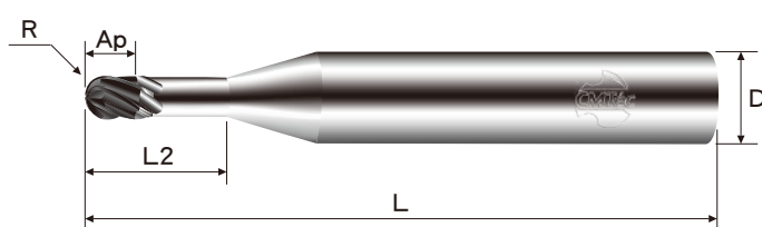
PCD球刀 | PCD Ball Nose End Mills
