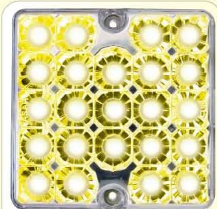
5564-23LED 透明殼黃燈 黃鑽石燈三線全亮型 5564-23LED Daytime yellow light, three lines, all-lit type
