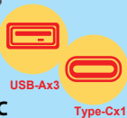
GK-UF/GK-UFQC Input range: 12V/24V USB-Ax3 : 5V/2.4A, 9V/2A, 12V/1.5A(18Wx3) USB-C : 5V/3A, 9V/3A, 12V/3A, 15V/3A, 20V/3A(60W)
